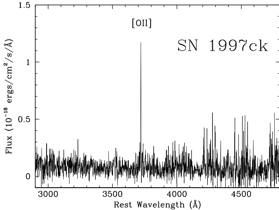
FIG. 1.—Identification spectra ( \ln f_{\lambda} ) of high-redshift SNe Ia. The spectra obtained for the 10 new SNe of the high-redshift sample are shown in the rest frame. The data are compared to nearby SN Ia spectra of the same age as determined by the light curves (see Table 1). The spectra of the three objects from Garnavich et al. (1998a) are also displayed.
